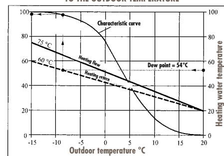
HEAT PRODUCTION ACCORDING TO THE OUTDOOR TEMPERATURE
