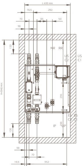
Model: Luna Sat RZH1-MB without casing
