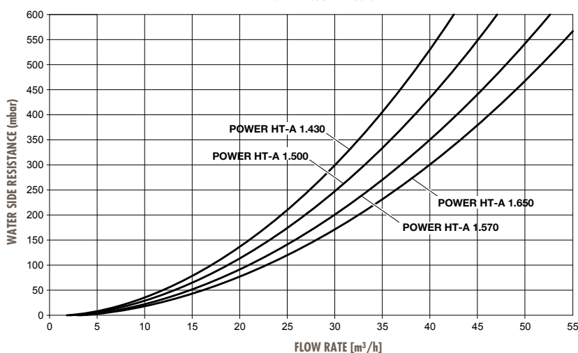
EXCHANGER PRESSURE LOSSES
