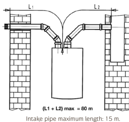
Installation example with horizontal dual flue ducts
