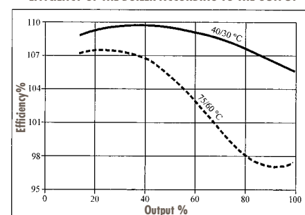
EFFICIENCY OF THE BOILER ACCORDING TO THE OUTPUT
